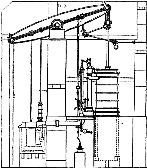
Fig. 199. A Cornish Pumping Steam-engine. (Bourne.)
